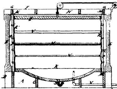
2235 Tiffany's Apparatus for Manufacturing and Storing Illuminating Gas.
