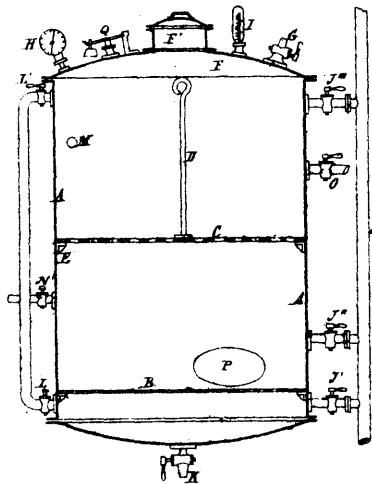
20779 Leplay's Apparatus for Baryta or Strontia Treatment of Saccharine Liquors, &c.
