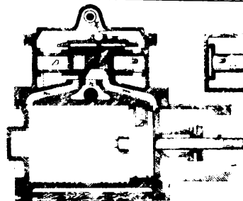
2618 Gilbert's Valve Motion.
