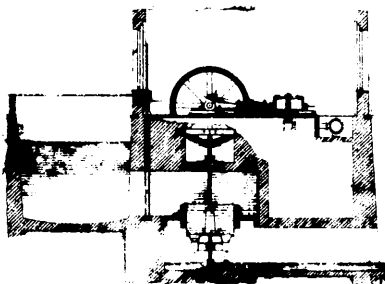
2623 Stanley's Hydro-pneumatic Motive Power.
