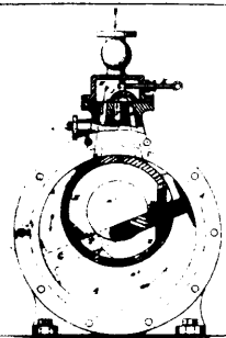
2628 Myers' Rotary Engine.
