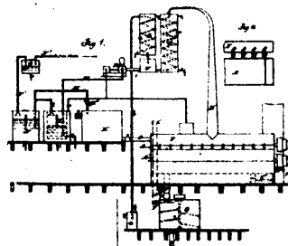
13508 Plumer's Process and Apparatus for the Manufacture of Fertilizers.
