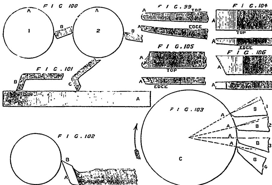
HARD TURNING TOOLS. —BRASS WORK. (See page 310.)
