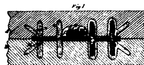
8633 Trickey's Spring Catch for Securing Blocks of Stone.
