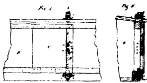
8607 Burtis' Seal Bolt for Car Doors.
