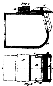
8638 Susemihl & Hewitt's Journal Oil Box Lid for Railway Cars.
