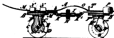
6958 Leggo's Improvements in Skates.
