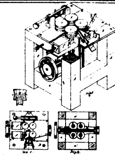
6949 Parker's Improvements on Hoop Shaving Machines.
