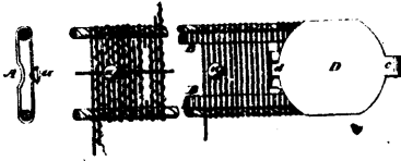
6189 Pulvermacher's Improvements on Volta-electric Appliances.
