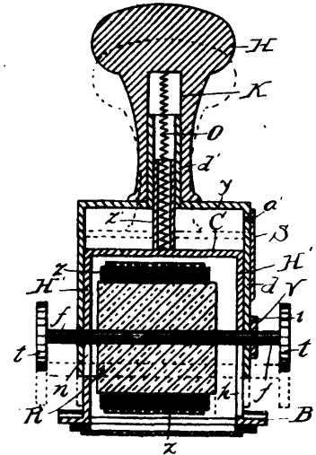
30948 Norrington's Hand Stamp.
