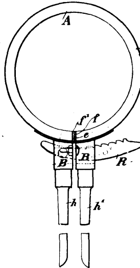
30947 Lawrence's Device for Stopping Leaking in Hose, etc.
