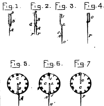
30950 Wesson's Medicine Dial.
