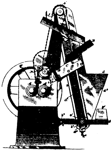
30942 Coleman's Mechanism for Feeding Nails, etc.
