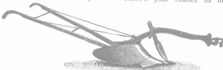
COCKSHUTT WALKING PLOW NUMBER 21
