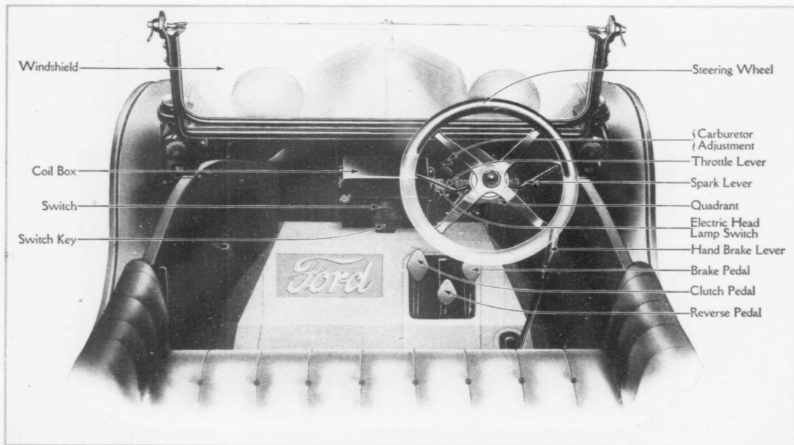
Ford Right Hand Control. (Cut No. 3)
