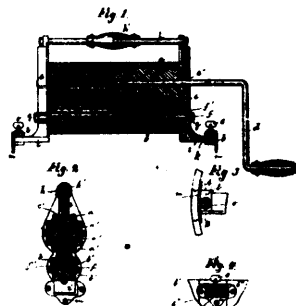
8190 Calef's Improvements on Washing Machines.
