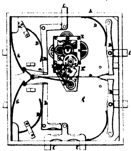
8178 Phillips' Improvements in Time Locks.
