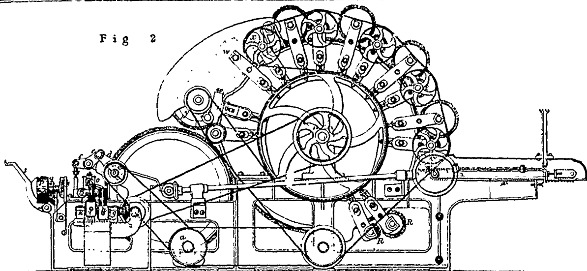
WOOL-CARDING MACHINERY.
