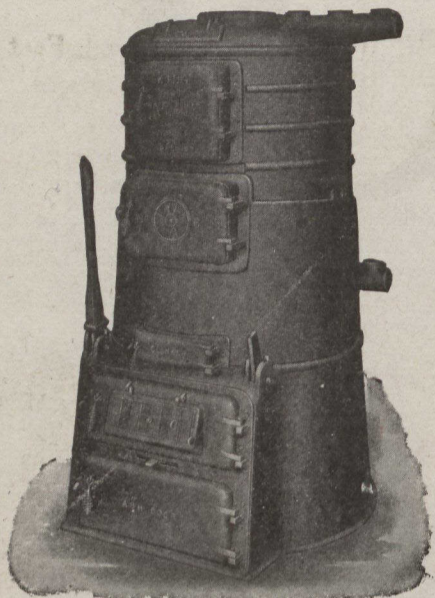
No. 6 High Base "King" Boiler, showing double shaker.
