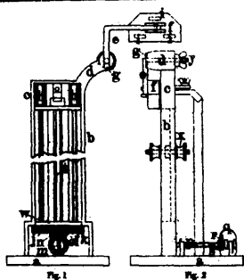
4065 Chapman's Saw-Sharpening Machine.
