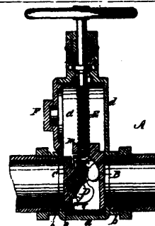
4070 Murdock's Stop Valves.
