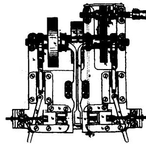
3350 Leopard's Machine for Making Railway Car-coupling Pins.
