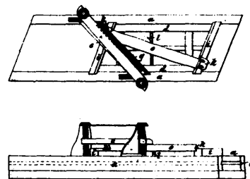
3340 Martin's Veneer Cutting Machine.
