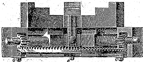
Fig. 1. Common Jaw.
