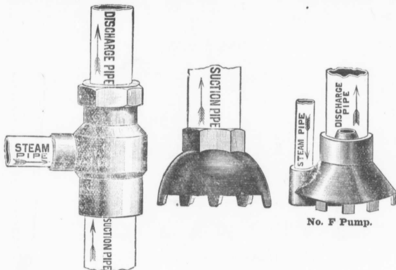
No. L Pump and Strainer.
