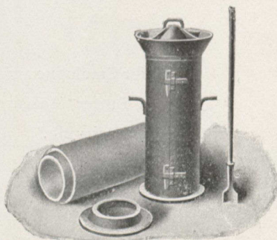
Moulds for Making Concrete Drain Tile
