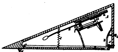
3743 Wetherhill's Portable Burglar Alarm.
