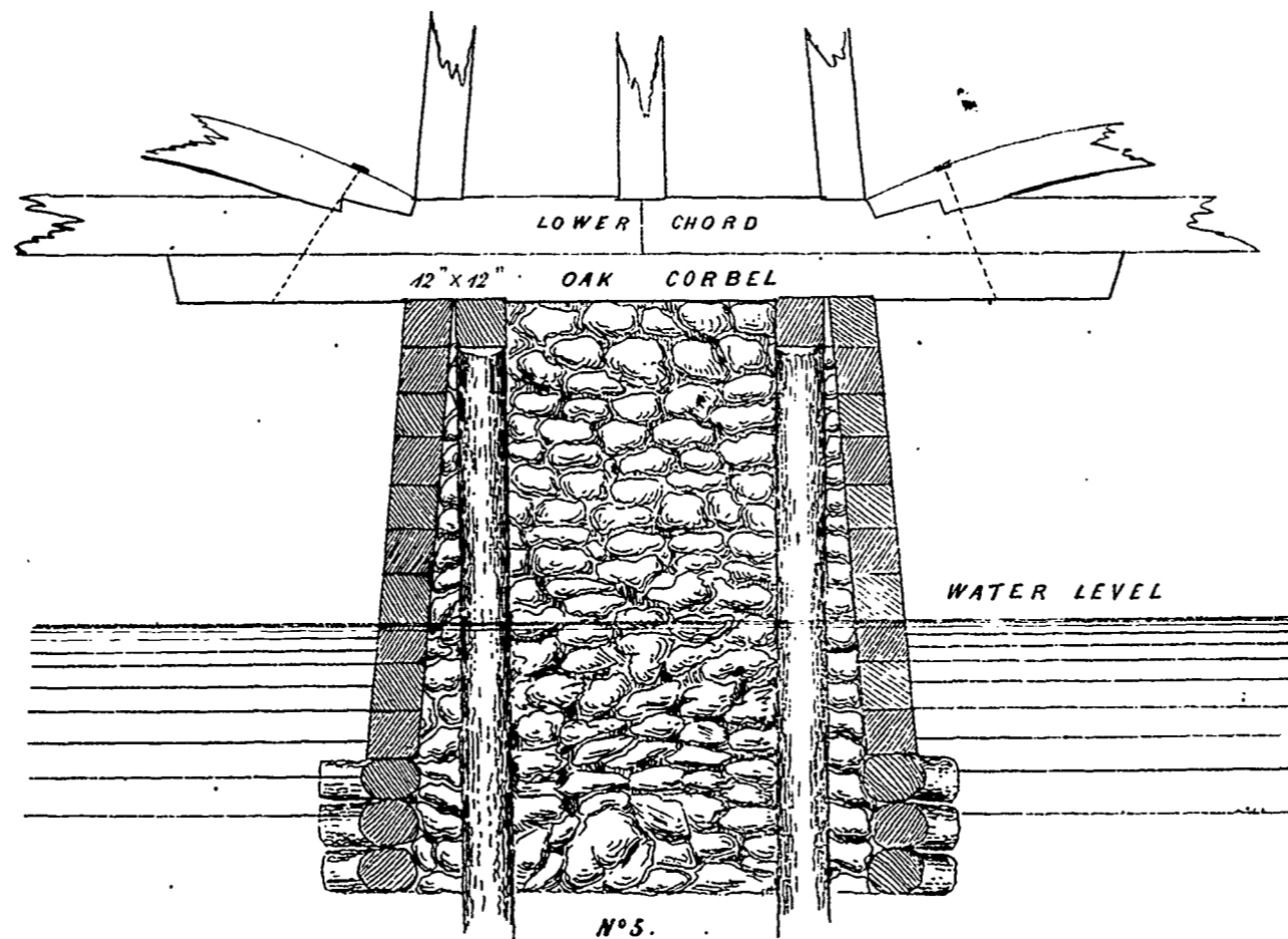
LONGITUDINAL SECTION OF PIER
