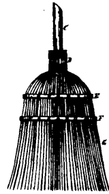
8798 Lay's Improvements on Brooms.
