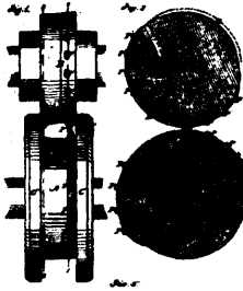
7774 Batchelder's Rolls for Making Horse Shoe Blanks.
