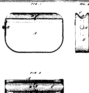
2107 Hunter & Foster's Tobacco Box and Cutter.
