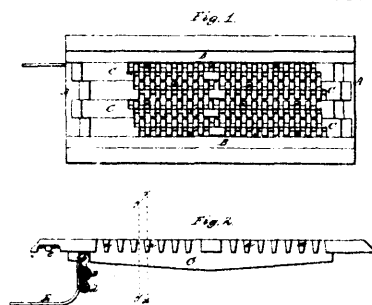
2108 Stanton's Grate Bar.
