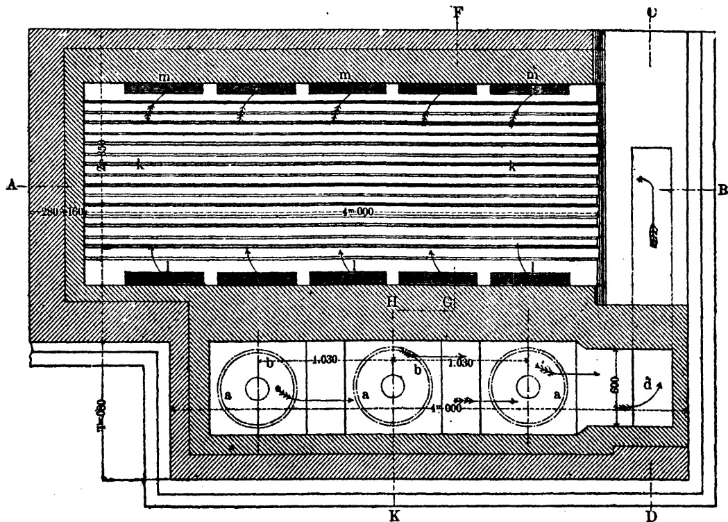
Bower Furnace for Coating Iron and Steel.—Fig.4.—Horizontal Section through Muffle, shown by L P in Fig. 2.
