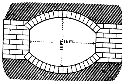
Worcester's Sewer.—Section of the Large Sewer in the City of Worcester, Mass.
