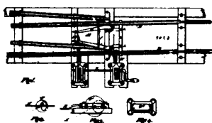
2306 Mercier's Self-Operating Railway Switch.
