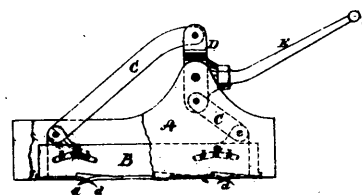
2308 Dann &amp; Swartwoort's Saw Mill Dog.
