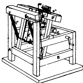
2298 Corney &amp; Turner's Stop Motion for Looms.
