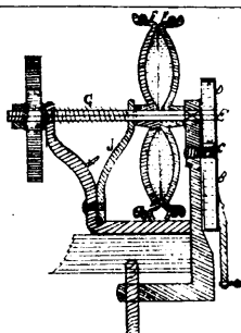
2309 Livergood's Machine for Sharpening and Cleaning Knives.
