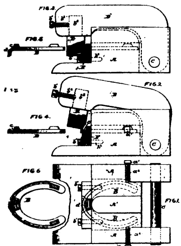
37440 Billings and Kirk's Machine for Forming Clips on Horse Shoes.
