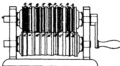
4388 Lewis & Mitchell's Horse-shoe Blank Rolling Machine.
