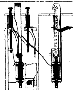
4386 Law's Improvements in the Millar Car-coupler.
