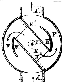
4385 Baldwin's Combined Radiator and Damper for Stove-pipes, &c.
