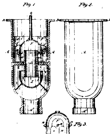
Baker's Water Trap.
