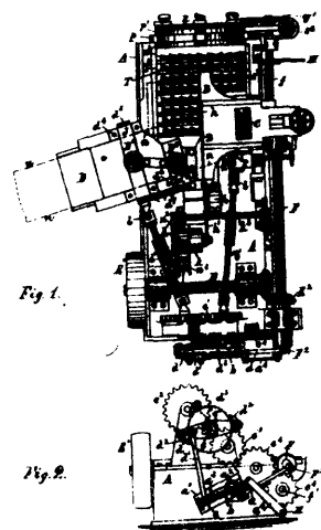
Green's Spiral Welding Machine.
