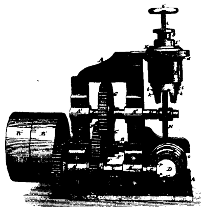
17352 Côté's Improvements in Machines for Shaping Boot and Shoe Counters.
