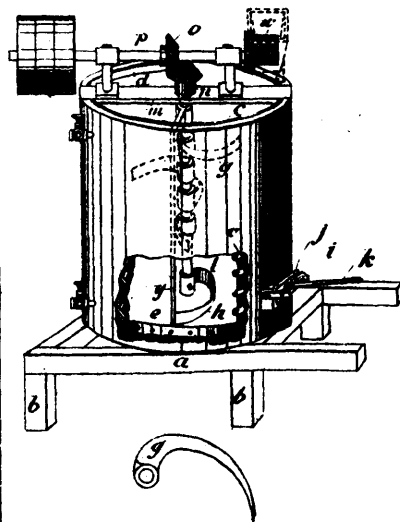
17360 Freeland's Improvements in Soap Making Machinery.
