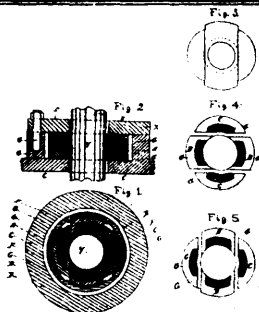
13432 Osgood & Monroe's Improvements on Metallic Packings.
