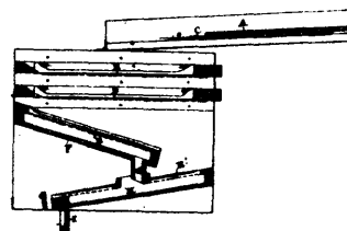
13442 Cavers's Improvements on Fanning Mills.
