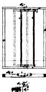
13441 Barnard's Improvements on Cattle Stand-bins.
