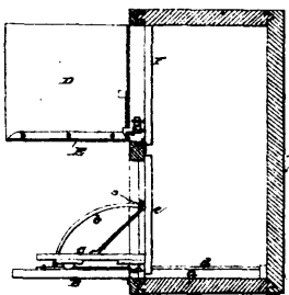
13435 Baldwin's Improvements on Refrigerators.
