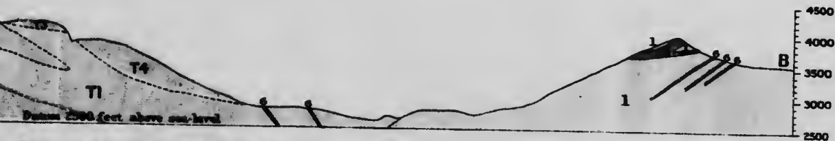
Structural section along line AB Scale, horizontal and vertical 2000 feet to 1 inch
