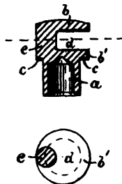
7558 Bray's Lacing Stud for Boots and Shoes.
