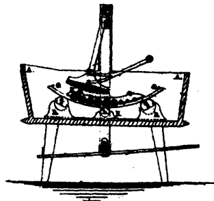
7560 Sault's Improvements in Washing Machines.
