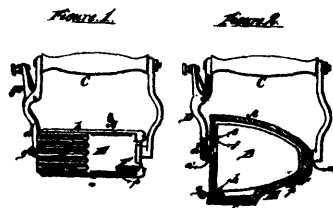
7547 McCausland's Improvements on Fluting and Sad Irons.
