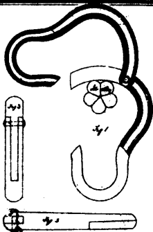
4581 Clements' Jib and Sail Hank.
