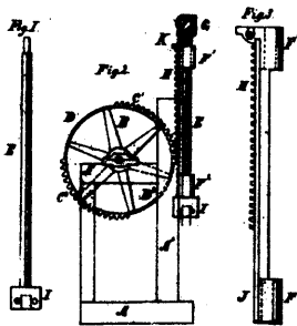
4592 Dagenais &amp; Brush's Rock Drill.
