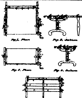
4585 Bouteb's Quilting Frame.
