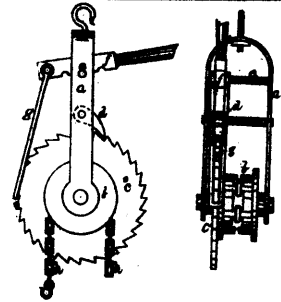
4588 Davis' Machine for Raising Stumps, &amp;c.
