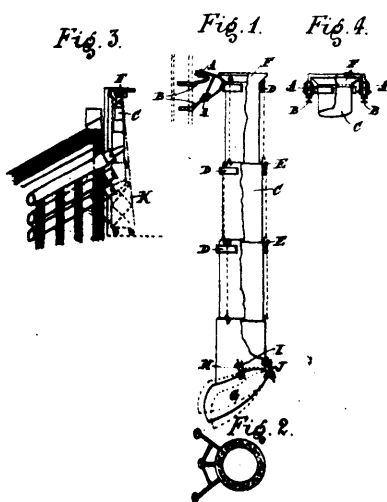
33795 Van Vestrant's Apparatus for Charging Gas Retorts.
