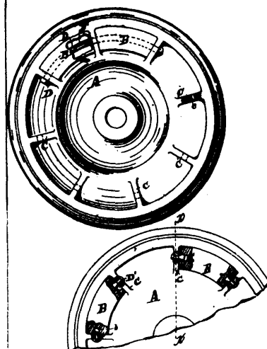
33797 Griffin's Car Wheel.
