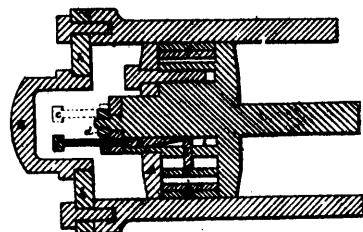
4795 Roberts, Pharis, Pharis, &amp; Laass's Method of Expanding Steam-Cylinder Packing Rings.
