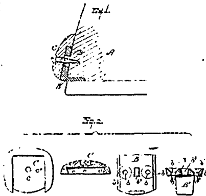
30048 Floyd's Toe Weight.
