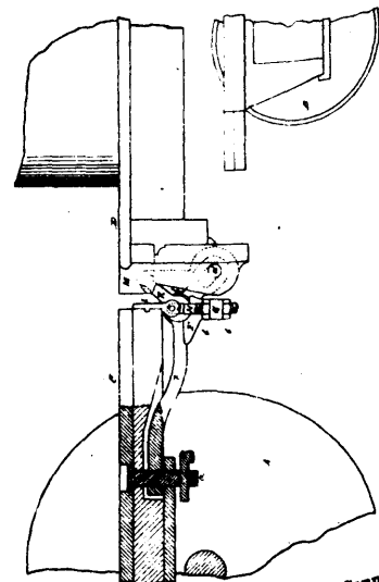
18688 Purves & Craven's Draw Bar for Connecting Locomotive and Tender.
