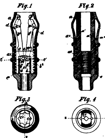
18690 Watson's Bit Brace.
