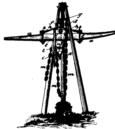
18685 Howe's Stump Machine.
