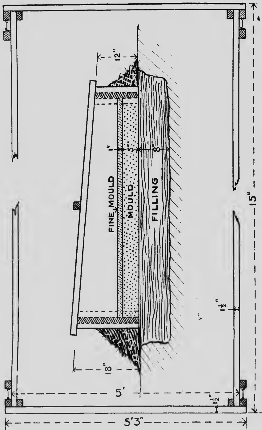
PLATE 1.—Graphic illustration of the construction of the semi-hot bed frame assembled and in place.
