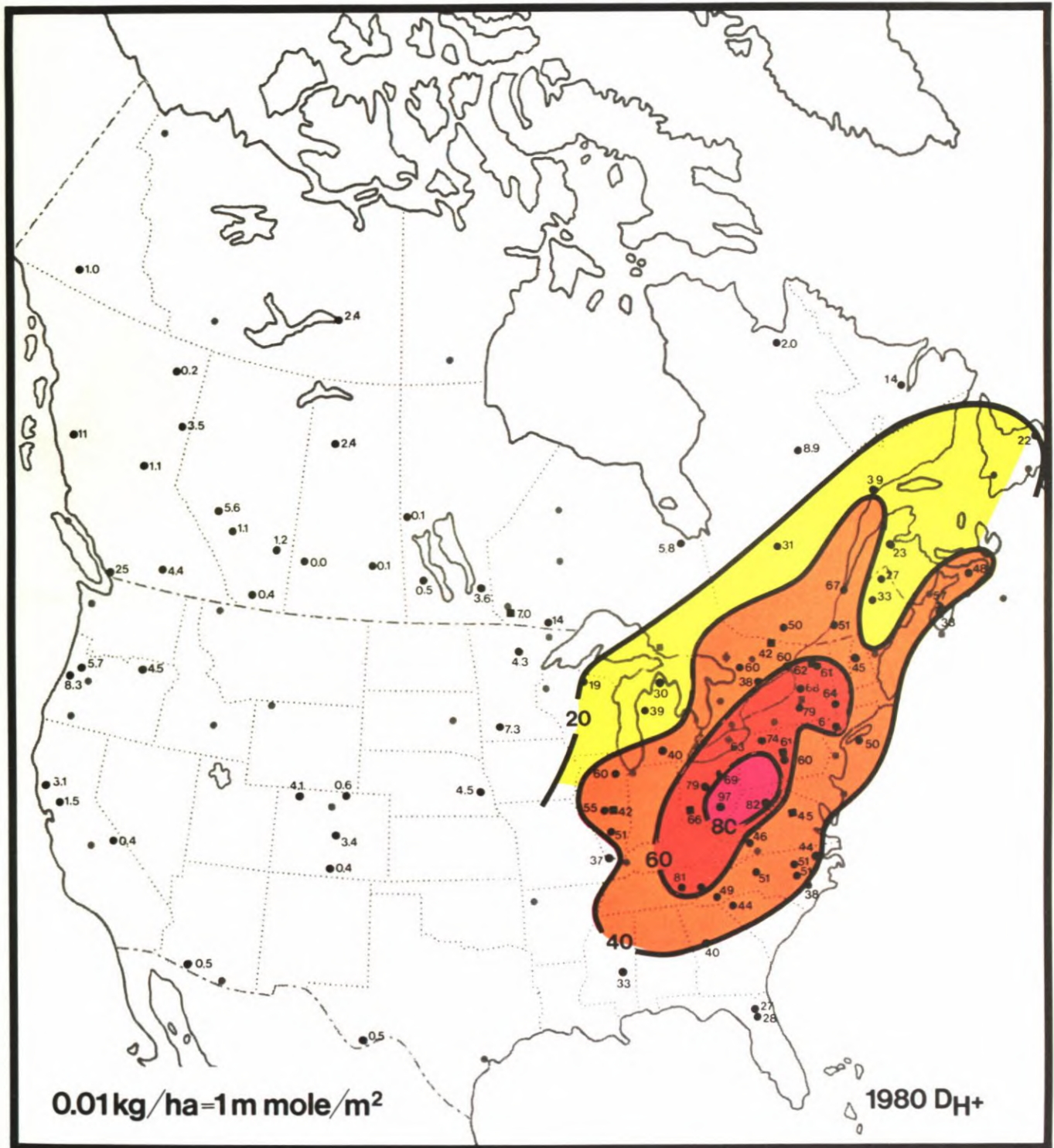
Precipitation amount- weighted mean hydrogen ion deposition for 1980 (m moles per square meter)
