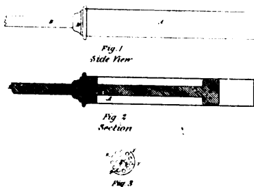
9232 Forrest's Improvements on Egg Beaters.
