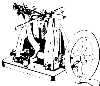
9233 Bugbee's Improvements on Saw Sets.
