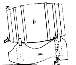
9234 Kirk's Improvements on Barrel Stands.
