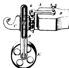
9243 Gale's Improvements on Plough Wheel Attachments.
