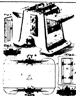
9238 Doane's Machine for Planing Wood.
