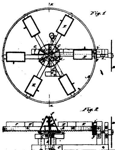
19624 Adkins' Horse Power.
