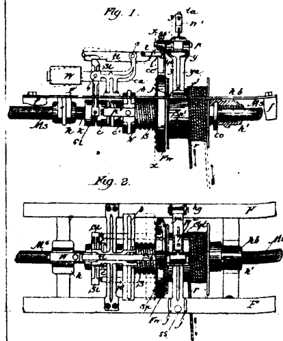
19619 Metcalf's Grain Shovel Mechanism.
