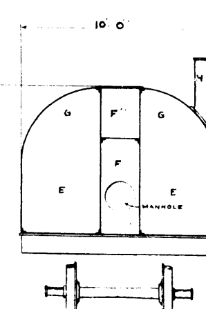
SECTION THRO' Y. Z. FIGURE 11.
