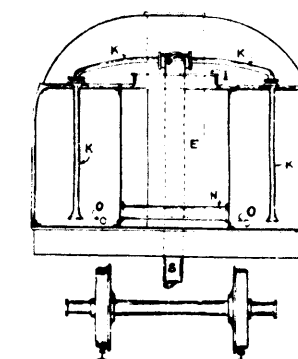
SECTION THRO' A. B. FIGURE 10.
