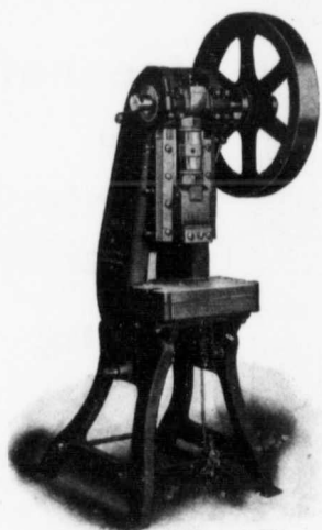
"BLISS" INCLINABLE POWER PRESS
