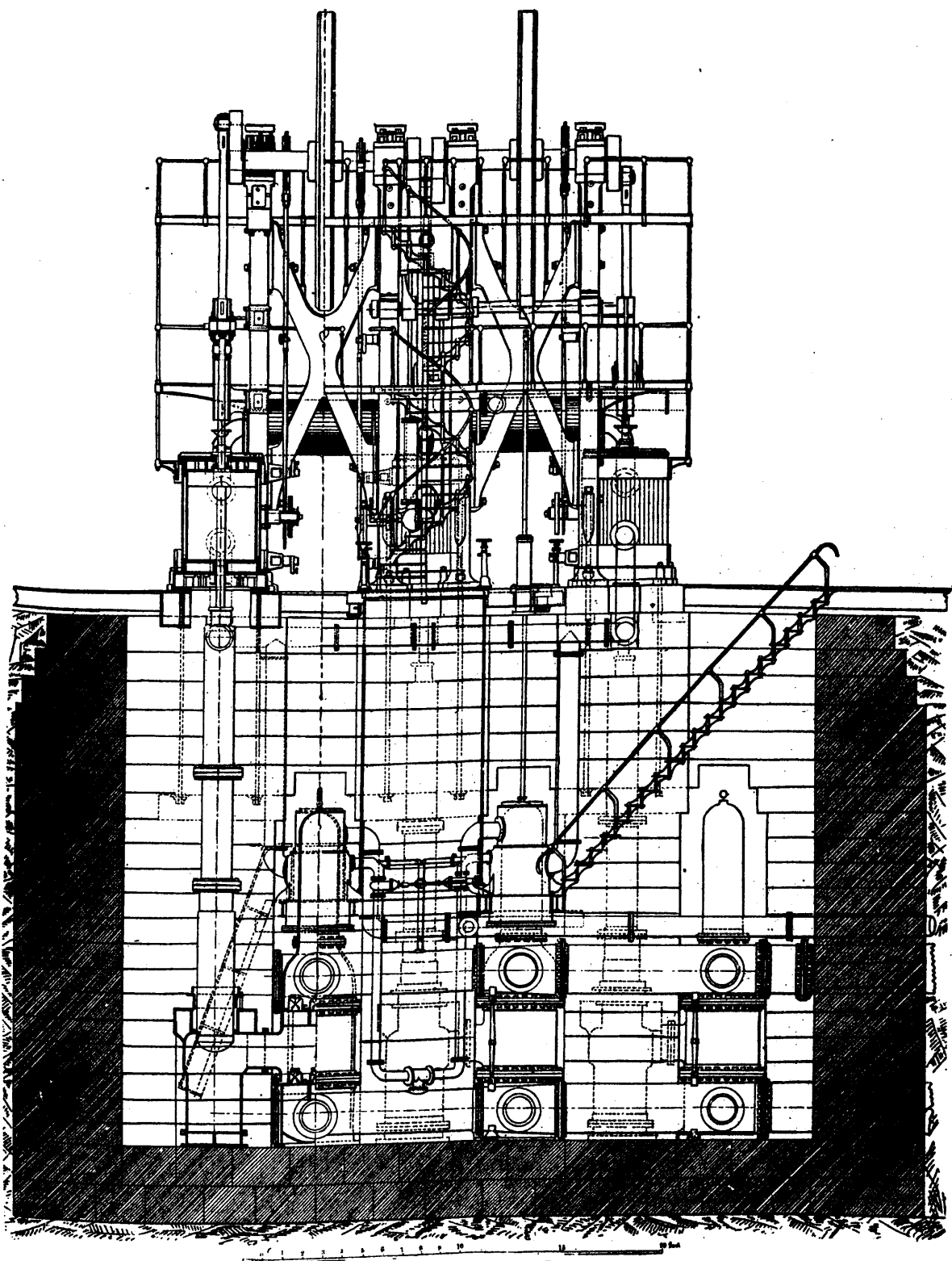
FIG. 2. SIDE ELEVATION OF ONE ENGINE.
