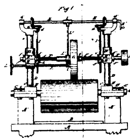
12183 LeRoy's Improvements on Attachment for Grinding Knives of Wood Planing Machines.
