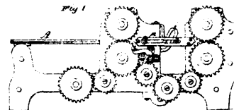
12172 Cross's Improvements in Paper Bag Machines.
