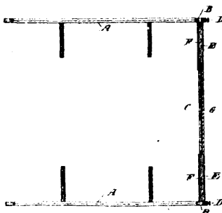
12188 Hensy's Improvements in Buggy Tops.
