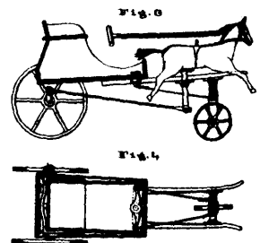
8574 Boss' Improvements on a Child's Wagon.
