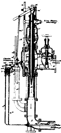
35224 Schutte's Automatic Condenser.
