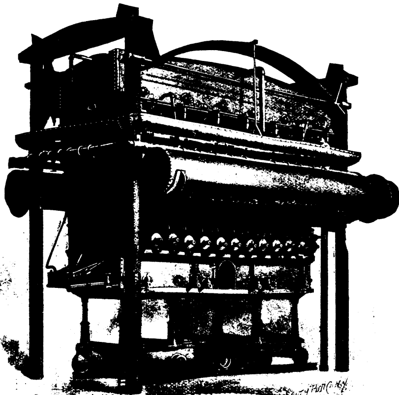
Modern Copper-Matting Furnace.
